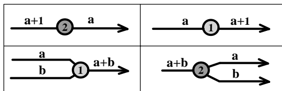
FIGURE 2. Bivalent and trivalent singularities and the 1-chain \tau_g(f) .
