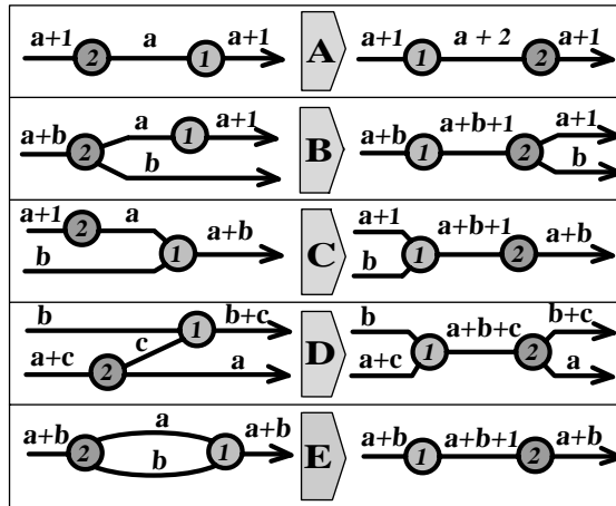
FIGURE 4. Generic patterns of moving a critical point of index 2 above a critical point of index 1 and the effect of these moves on the genera of fiber components.
