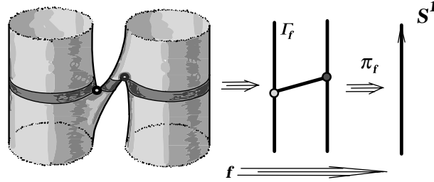
FIGURE 16. Attaching a slanted 1-handle.
