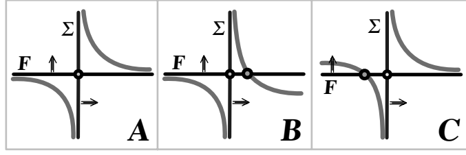
FIGURE 12. Three ways of resolving the intersection.
