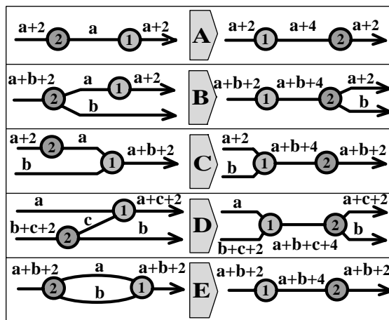
FIGURE 5. Generic patterns of moving a critical point of index 2 above a critical point of index 1 and the effect of these moves on the \chi_- -characteristics of the fiber components.
