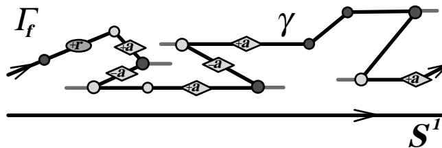
FIGURE 8. \int_\gamma [A] = \int_\gamma [R] .
