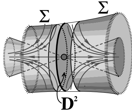
FIGURE 9. Moving \Sigma above the critical level of index 2 after a 2-surgery.
